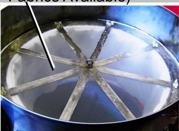
Interchangeable Screen Frames (Custom Meshes & Fabrics Available)
