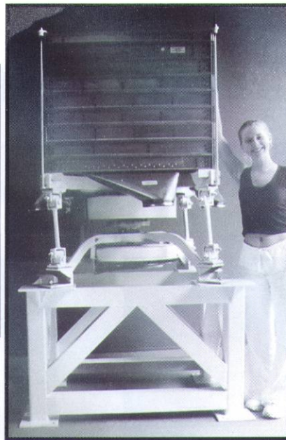
7 deck multiple separation gyratory sifter
